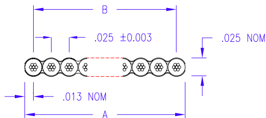
CROSS SECTION THRU FLAT
