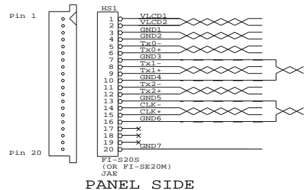
PANEL SIDE
