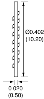
WASHER
