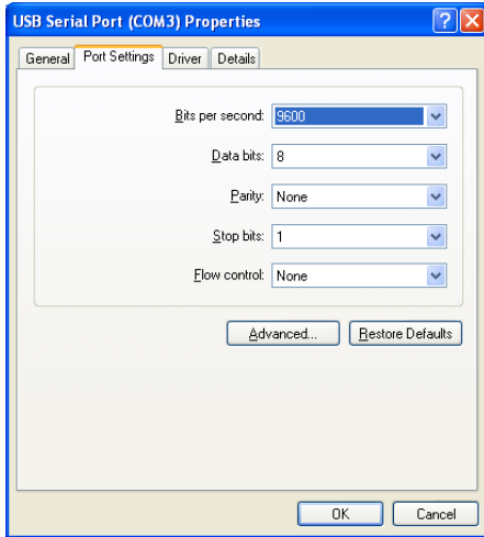
Figure 3-5 Settings Tab
