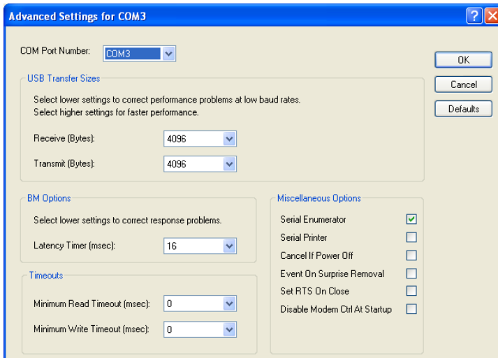
Figure 3-6 Advanced Options
