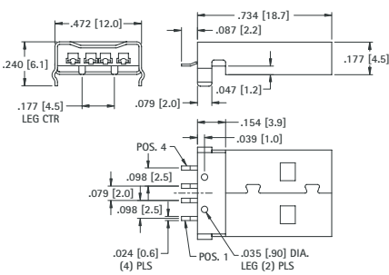
Mounting Detail
