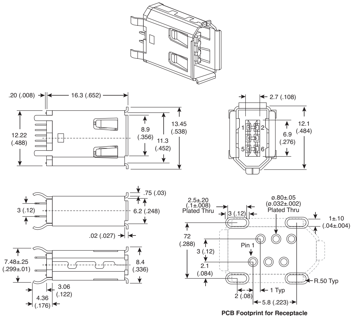
PCB Footprint for Receptacle
