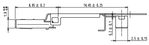
Fig-2 COMPONENT BREAK OFF FIGURE (FREE)
