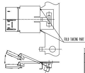
Fig-2 COMPONENT BREAK OFF FIGURE (FREE)
