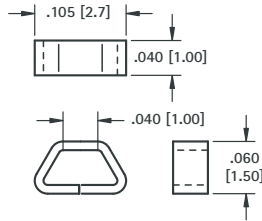
Pad Layout
