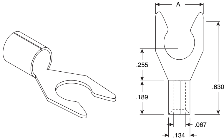
Dimensions In.
