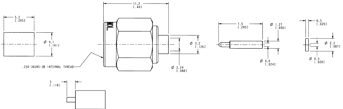
RECOMMENDED CABLE STRIPPING DIMENSIONS SCALE 3.000
