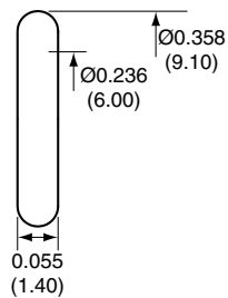
O-RING
