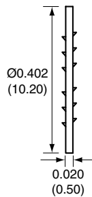
WASHER
