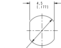
RECOMMENDED MOUNTING HOLE DIM'S. SCALE 5.000
