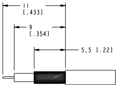
RECOMMENDED CABLE STRIPPING DIM'S. SCALE 3.000
