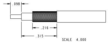
TRIMMING DIMENSIONS FOR RG-58 CABLE
