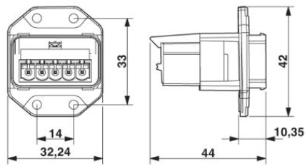
Push-Pull MSTB-Anbaurahmen
