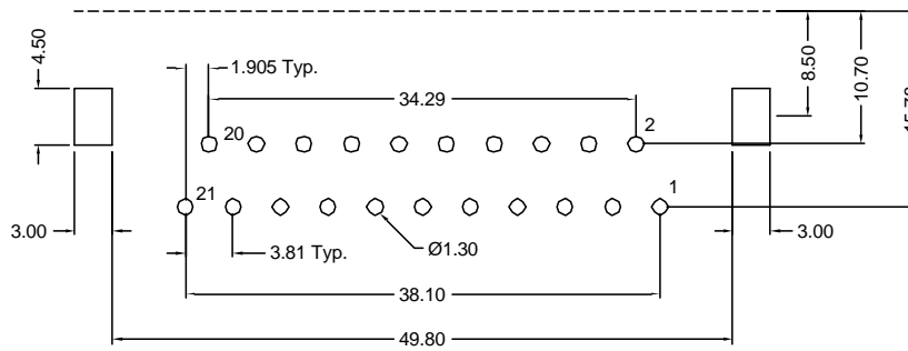
Recommended PCB Layout (Bottom View)
