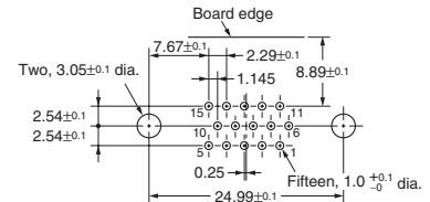
Mounting holes (t = 1.6 mm, bottom view)
