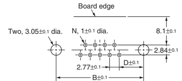
Mounting holes (t = 1.6 mm, bottom view)
