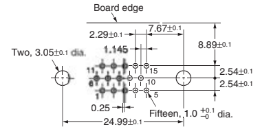
Mounting holes (t = 1.6 mm, bottom view)
