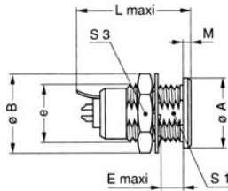
ERN Fixed socket, nut fixing, with earthing tag
