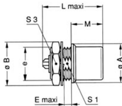
EHP Fixed socket, nut fixing, protruding shell
