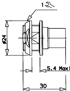
HG : Sealed Front Mount Receptacle
