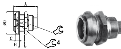
EA: Double Nut
