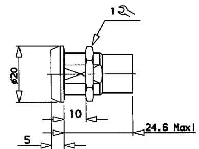
HM : Sealed Rear Mount Receptacle
