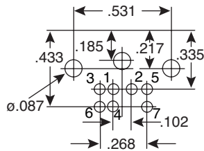
7-Pin 161-2307
