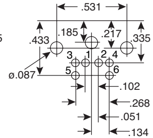
6-Pin 161-2306
