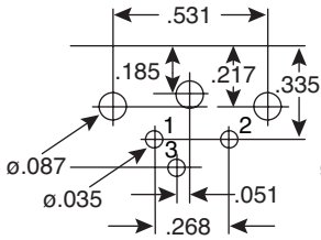
3-Pin 161-2303
