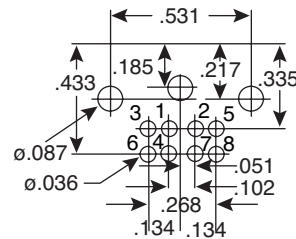
8-Pin 161-2308
