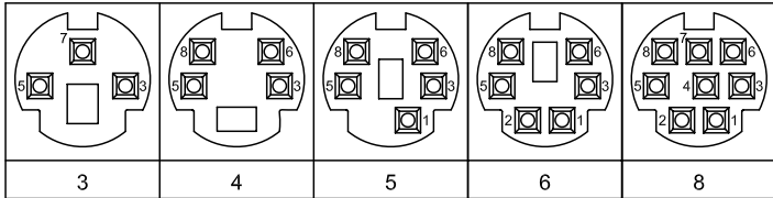
Recommended PCB Layout (Top View)
