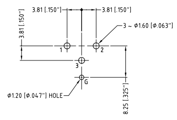
PCB - LAYOUT COMPONENT SIDE TOLERANCE: ±0.05mm [0.002\"/>
