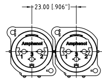
MIN MOUNTING PITCH SCALE 1:1
