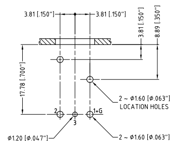
PCB - LAYOUT COMPONENT SIDE TOLERANCE: ±0.05mm [0.002\"/>
