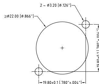
PANEL CUT OUT REAR VIEW
