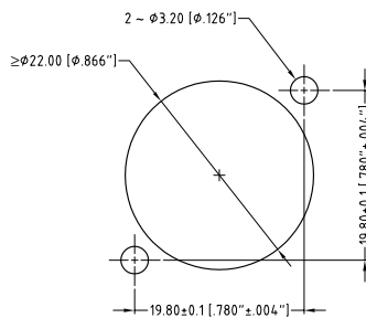
PANEL CUT OUT REAR VIEW
