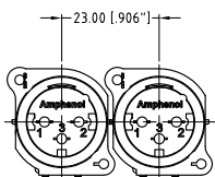
MIN MOUNTING PITCH SCALE 1:1
