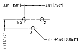
PCB - LAYOUT COMPONENT SIDE TOLERANCE: ±0.05mm [002"]
