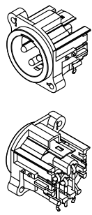
ISO VIEW SCALE 1:1
