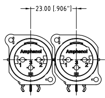
MIN MOUNTING PITCH SCALE 1:1
