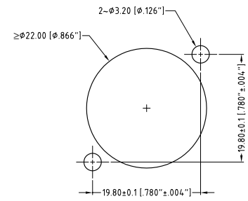
PANEL CUT OUT REAR VIEW
