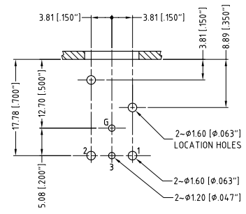
PCB - LAYOUT COMPONENT SIDE TOLERANCE: ±0.05mm [0.002\"/>
