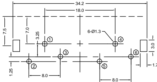
Recommended PCB Layout (Bottom View)
