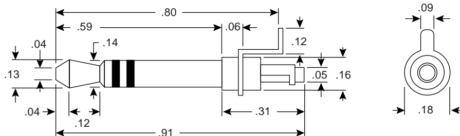
DIMENSIONS (IN)
