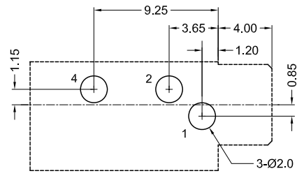
Recommended PCB Layout (Bottom View)
