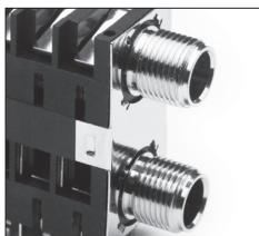
1/4" Shielding Plate
