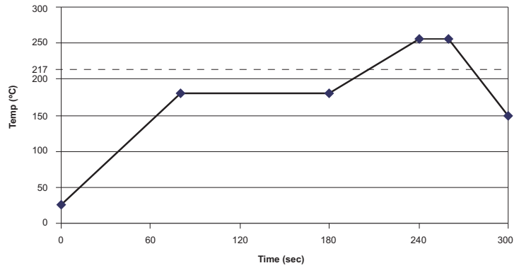
Lead Free Reflow Profile
