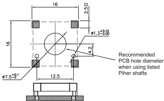
FOOT - PRINT
