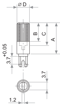
Hollow model shafts
