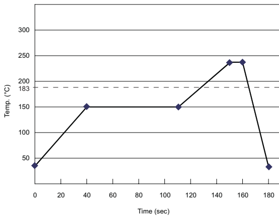
SnPb Reflow Profile
