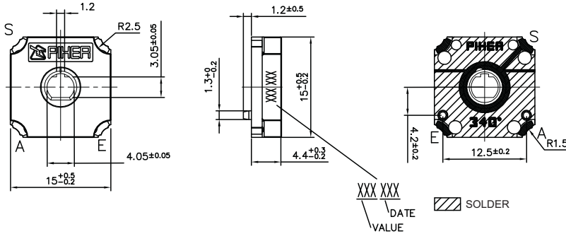
FOOT - PRINT
