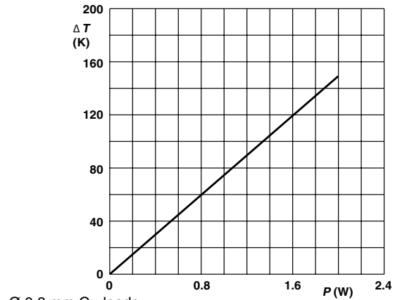
Ø 0.8 mm Cu-leads PR02 Hot-spot temperature rise ( \Delta T ) as a function of dissipated power.
