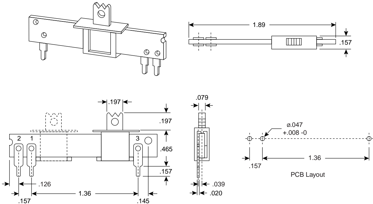
Dimensions (In.)
