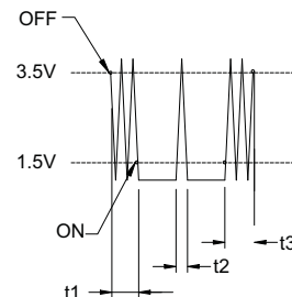
BOUNCE / CHATTER (FIG.3)
