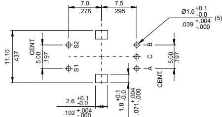
MOUNTING HOLE DETAIL VIEWED FROM MOUNTING SIDE
