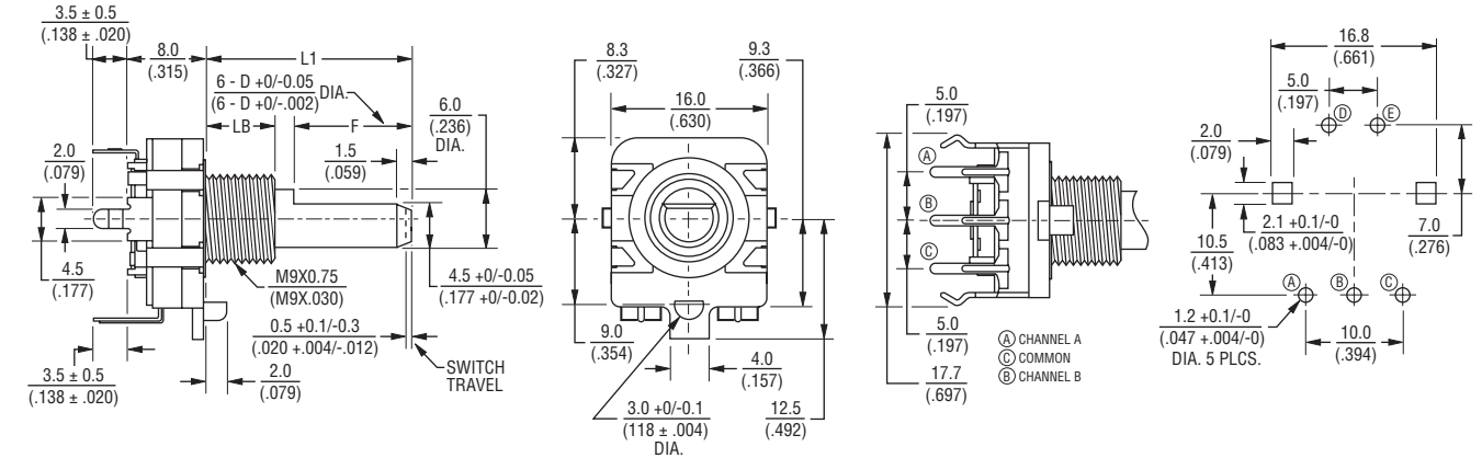
PEC16-4xxxF-Sxxxx
