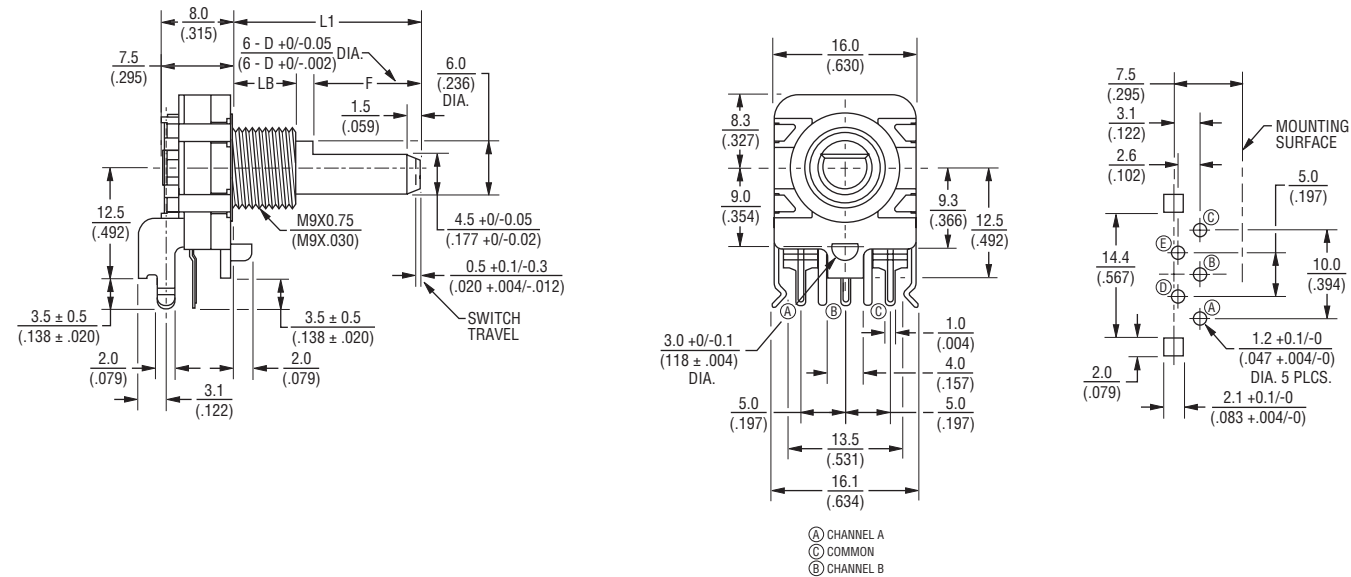
PEC16-4xxxF-Sxxxx
