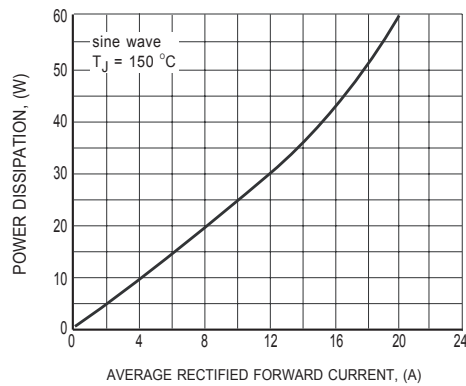
FIG.2 POWER DISSIPATION
