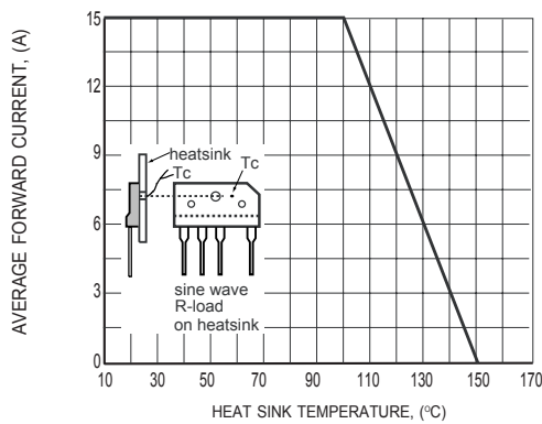
FIG.5 TYPICAL FORWARD CURRENT DERATING CURVE
