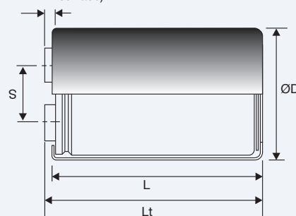
ALS30 Clamp Mounting
