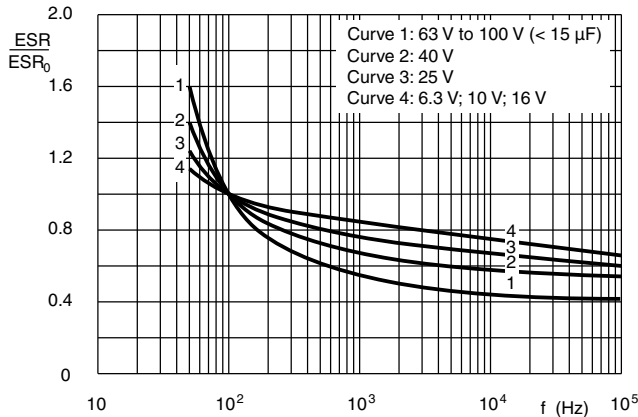
Case Ø D x L = 6.5 mm x 18 mm to 10 mm x 25 mm ESR 0 = typical at 20 °C, 100 Hz
