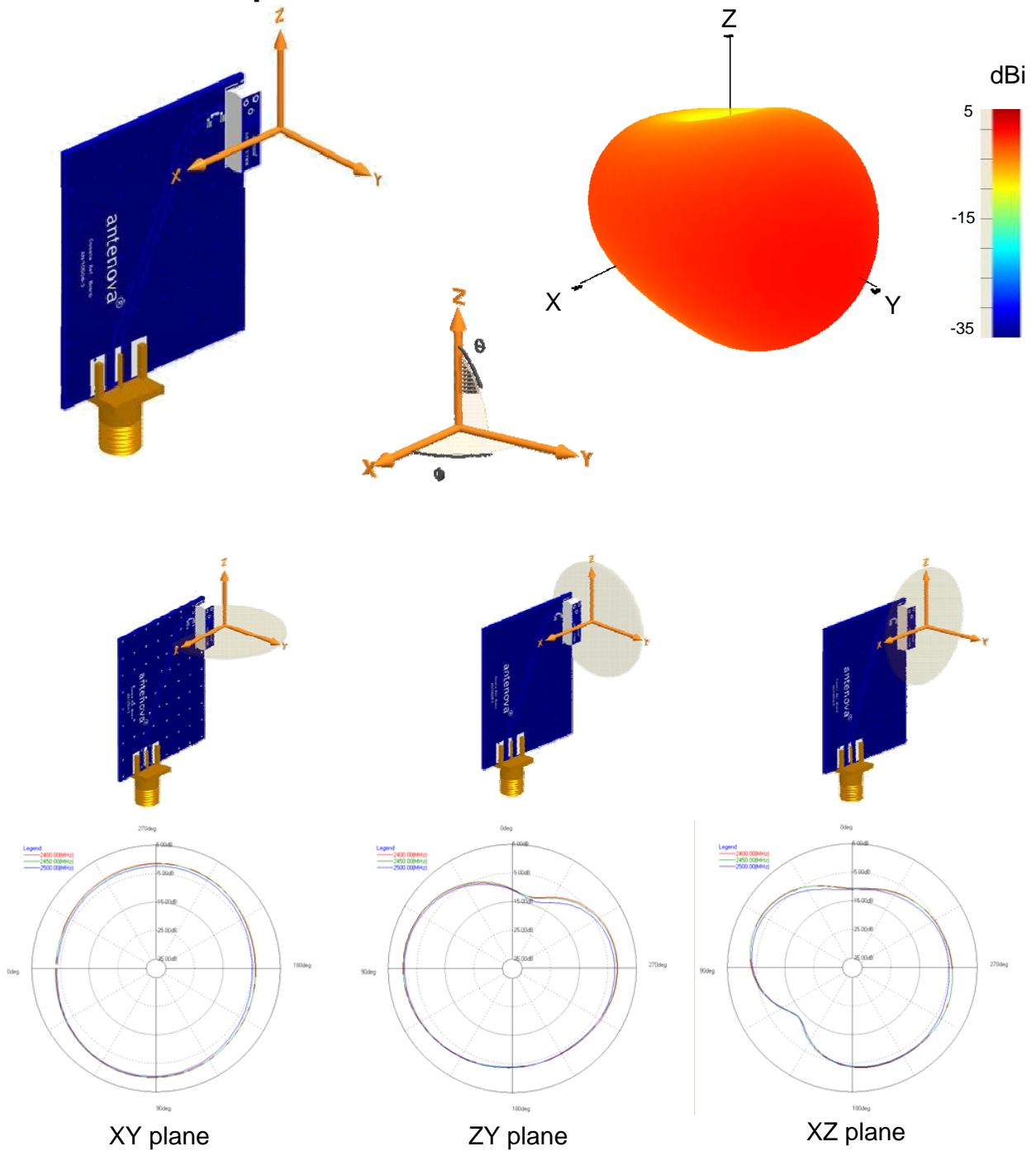
Patterns show combined polarisations measured on reference board A6111-U1
