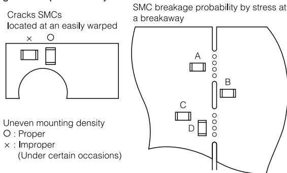
Fig.3 Component Layout
