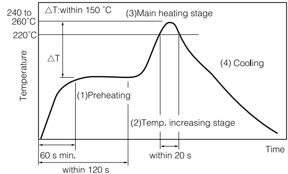
Fig.7 Recommended Soldering Temperature-Time Profile (Reflow Soldering)
