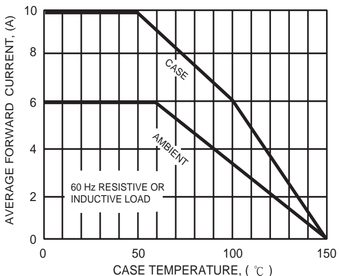
FIG. 2 - TYPICAL FORWARD CURRENT DERATING CURVE
