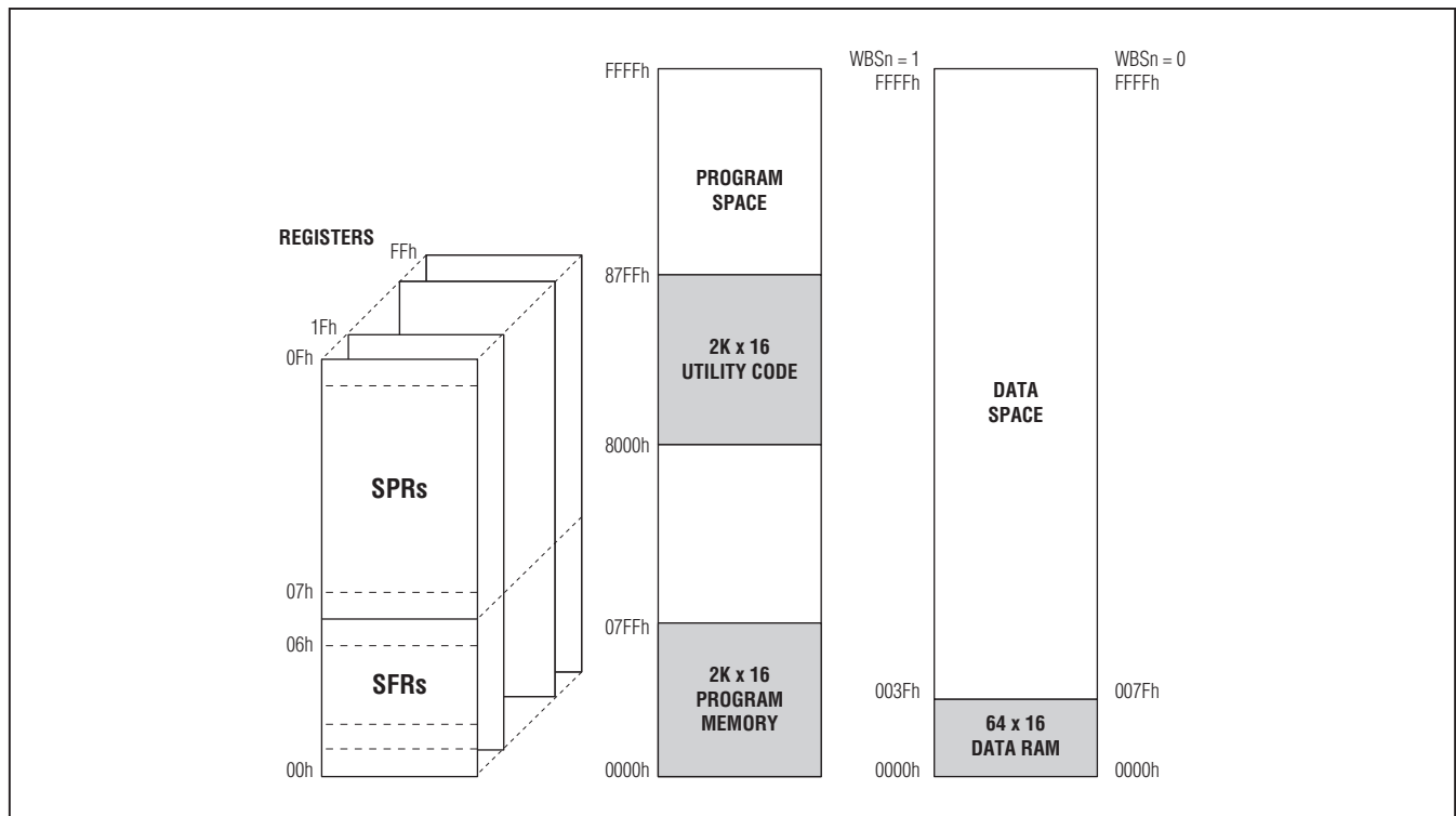
Figure 3. Memory Map
