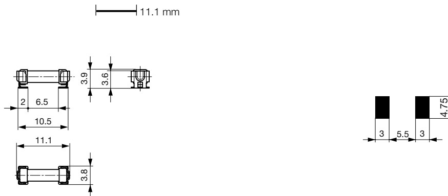
Soldering pads
