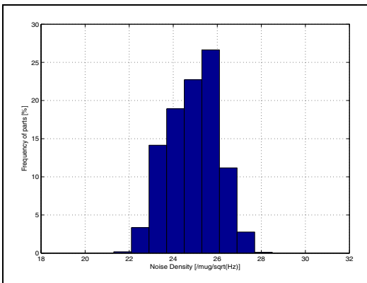
Figure 19. Noise density at 3.3 V (X, Y axis)
