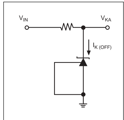
Figure 4. Test Circuit for I_{K(OFF)}
