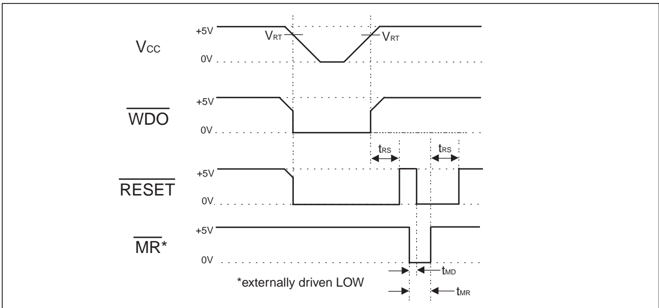
Figure 15. SP705/706 Timing Diagrams with \overline{WDI} Tri-stated. The SP707/708/813L \overline{RESET} Output is the Inverse of the \overline{RESET} Waveform Shown.
