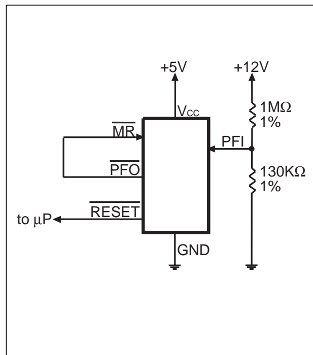
Figure 17. Monitoring Both +5V and +12V Power Supplies
