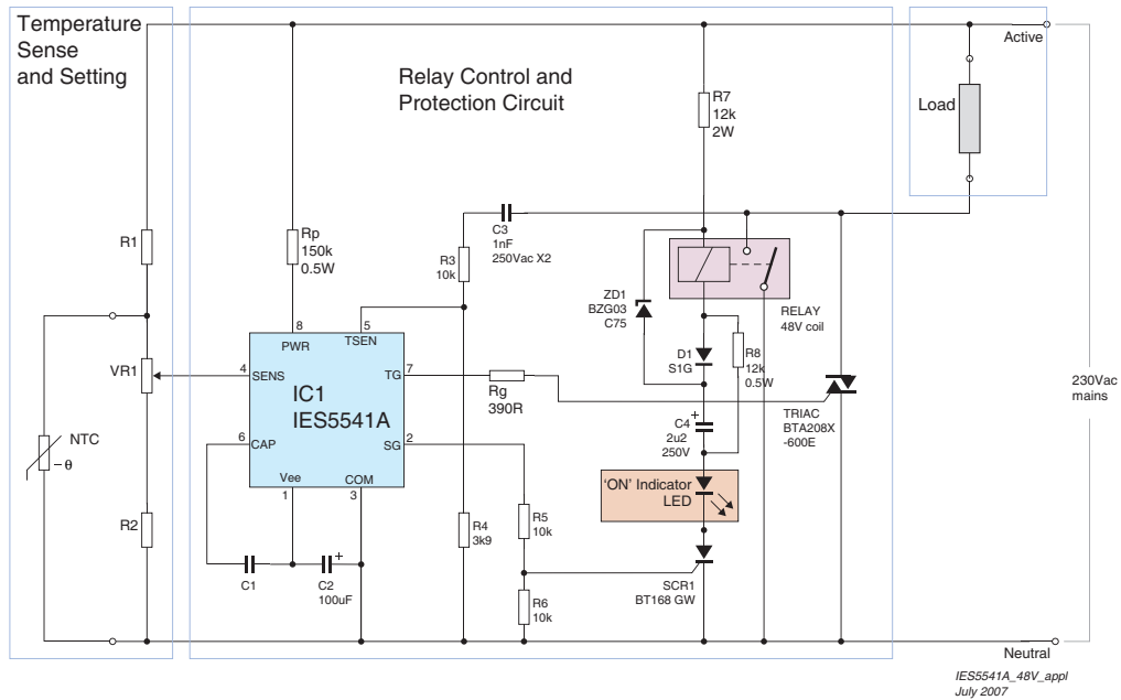
Fig.8 IES5541A application diagram: alternative relay drive for 48V relays
