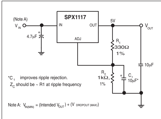
Figure 23. Improving Ripple Rejection
