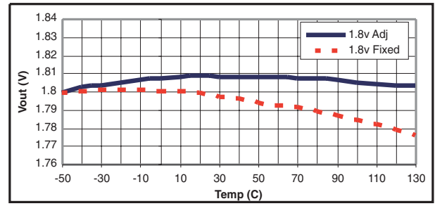
Figure 8. V_{IN}=3.3V , I_{OUT}=10mA
