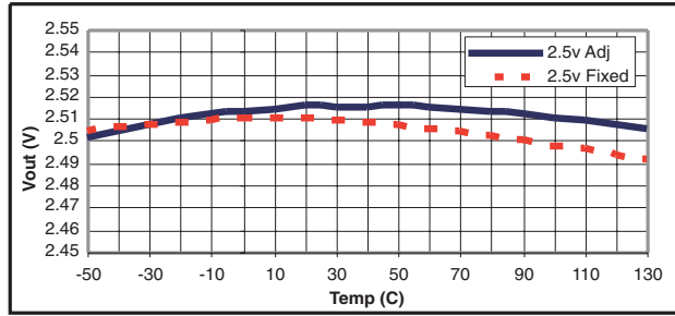
Figure 9. V_{IN}=4.0V , I_{OUT}=10mA
