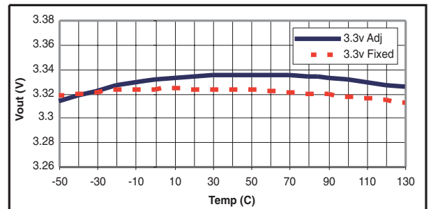
Figure 12. V_{IN}=5.0V , I_{OUT}=10mA
