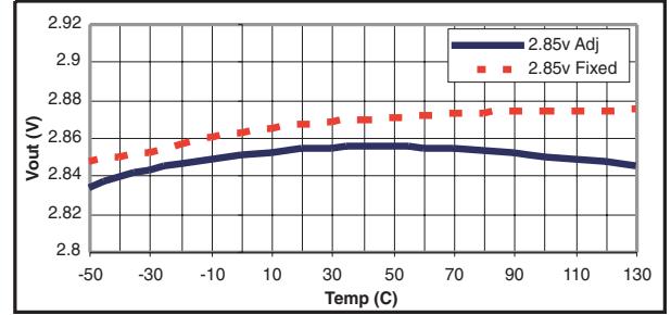
Figure 10. V_{IN}=4.85V , I_{OUT}=10mA
