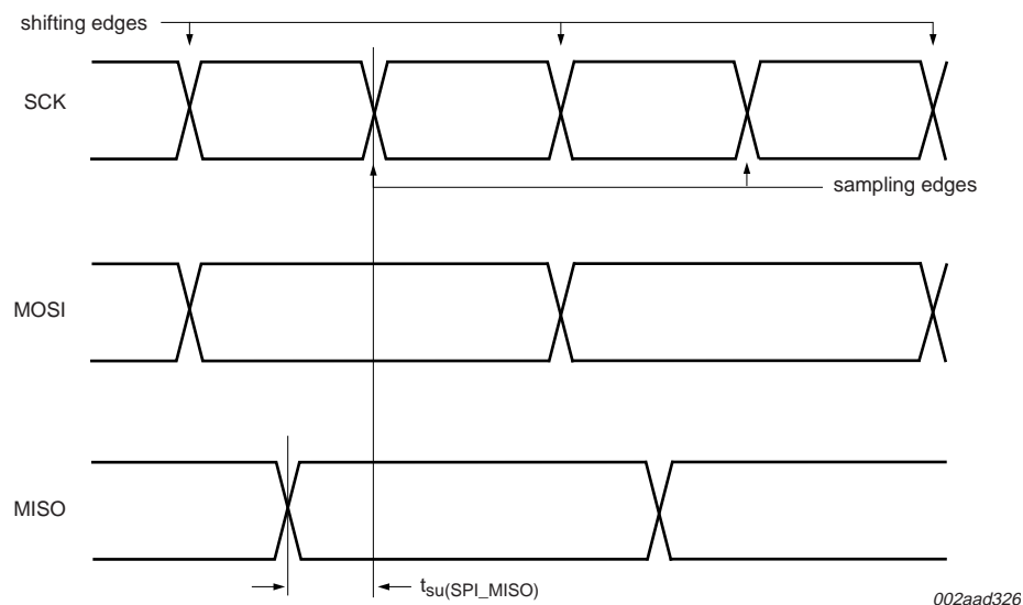
Fig 19. SSP MISO line set-up time in SPI Master mode
