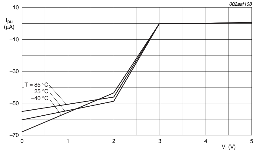
Fig 12. Typical pull-up current I_{pu} versus input voltage V_i
