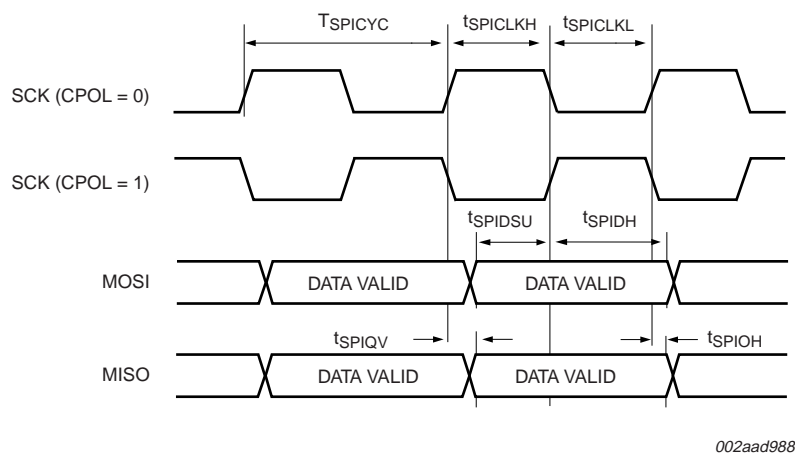
Fig 23. SPI slave timing (CPHA = 1)
