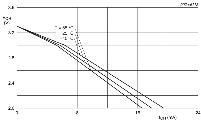
Fig 10. Typical HIGH-level output voltage V_{OH} versus HIGH-level output source current I_{OH}
