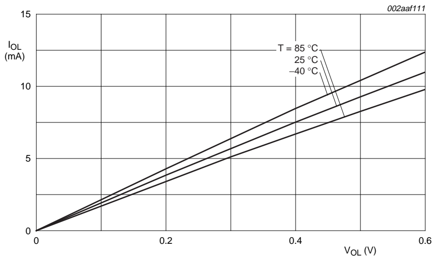
Fig 11. Typical LOW-level output current I_{OL} versus LOW-level output voltage V_{OL}
