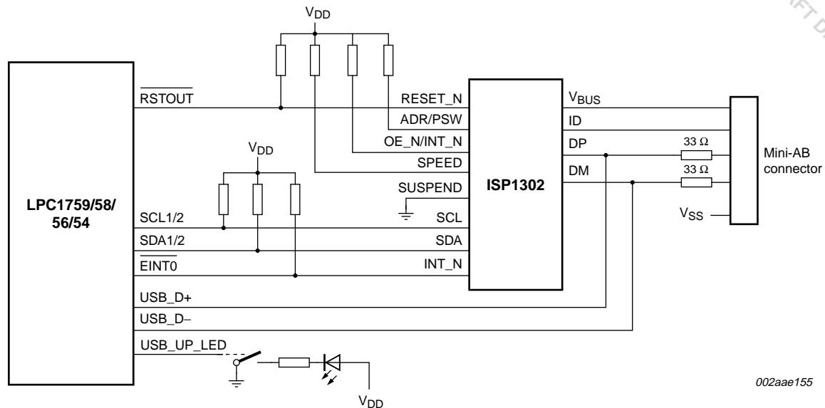
Fig 29. LPC1759/58/56/54 USB OTG port configuration
