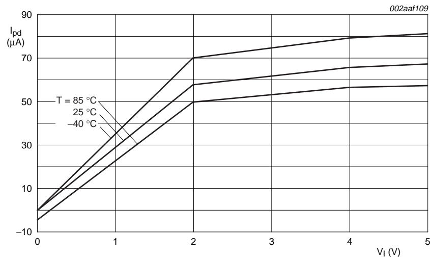
Fig 13. Typical pull-down current I_{pd} versus input voltage V_i
