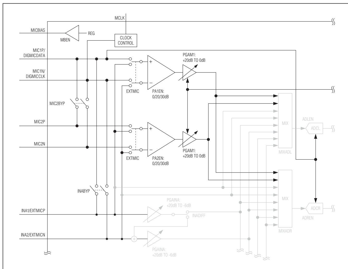
Figure 6. Microphone Input Block Diagram
