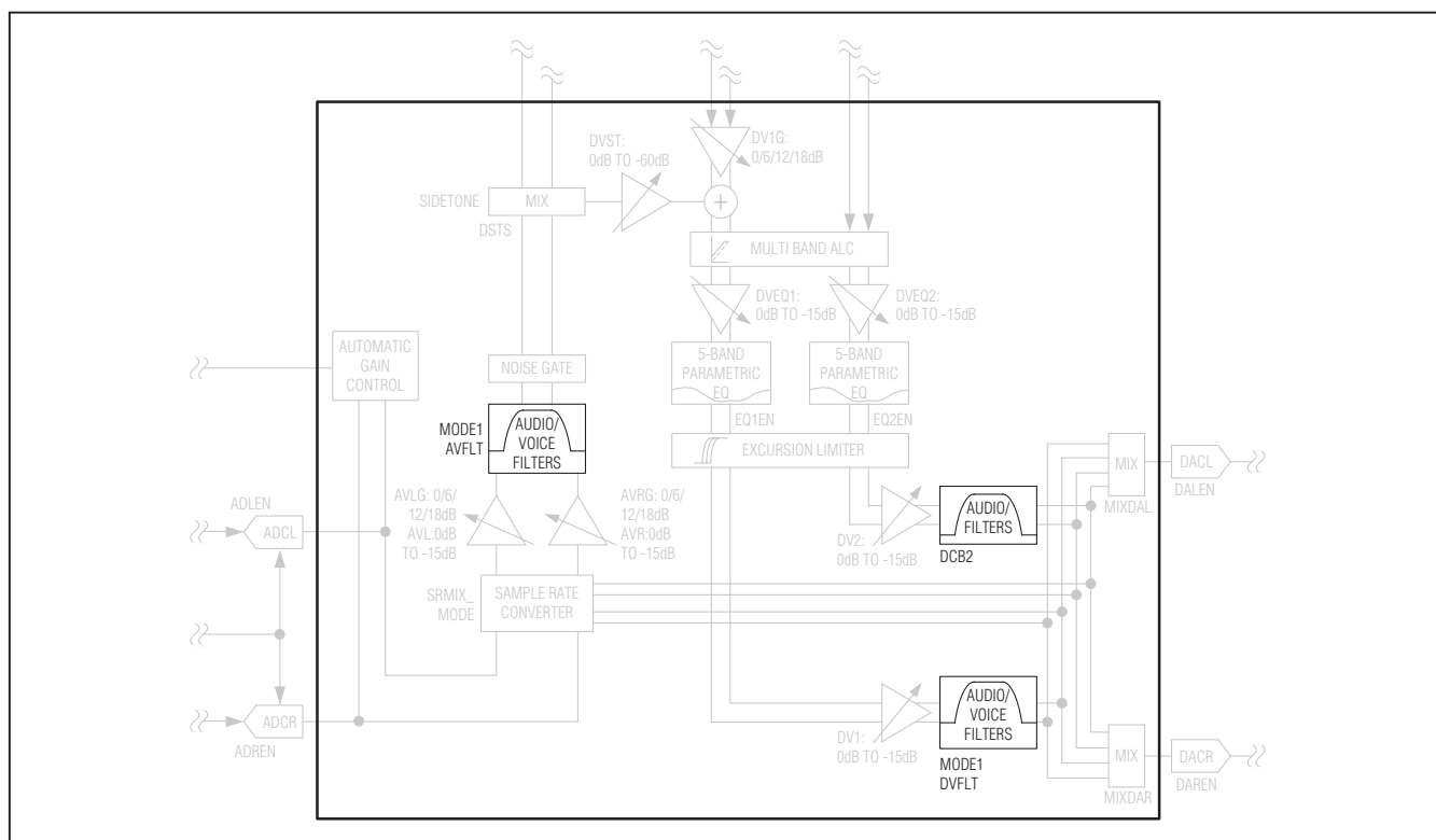
Figure 19. Digital Passband Filtering Block Diagram
