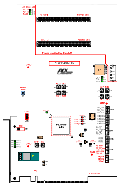
Figure 10. PEX8649-16U16D AIC RDK
