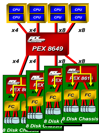
Figure 9. N+1 Failover.
