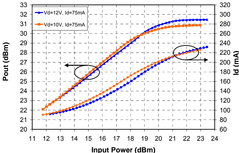
Power tuned data at 10GHz
