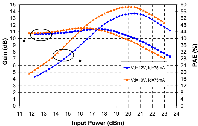
Efficiency tuned data at 10GHz
